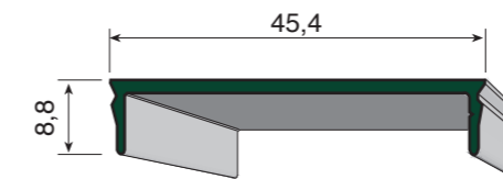
B/ 106 Grapa barandilla B102 cristal
