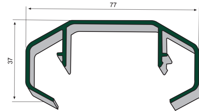
B/ 107 Pasamano hexagonal cristal
