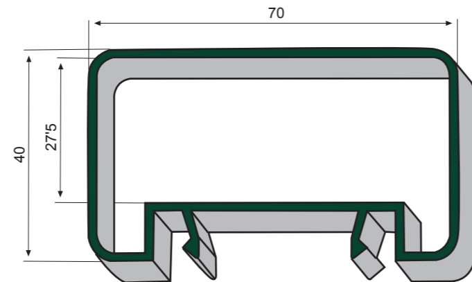
B/ 574 Pasamano rectangular
